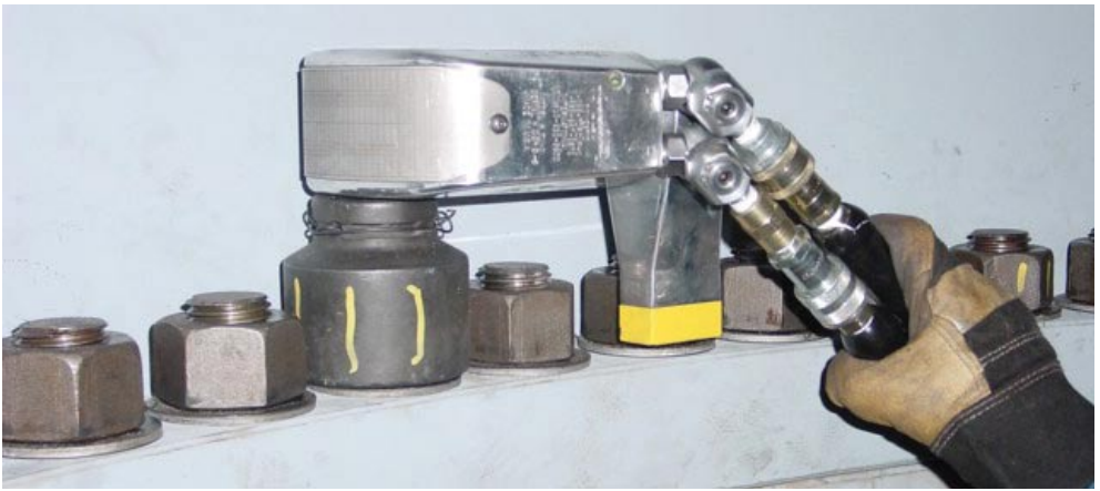
Fig. 6: The TorcUP TU device for windmills.
